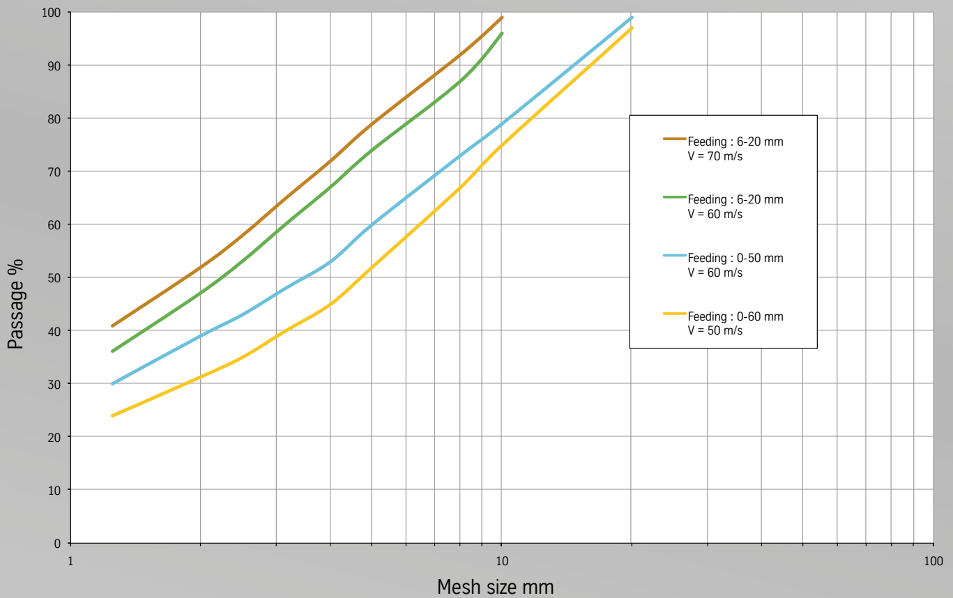
Limestone - PKV with two rows of blow bars
